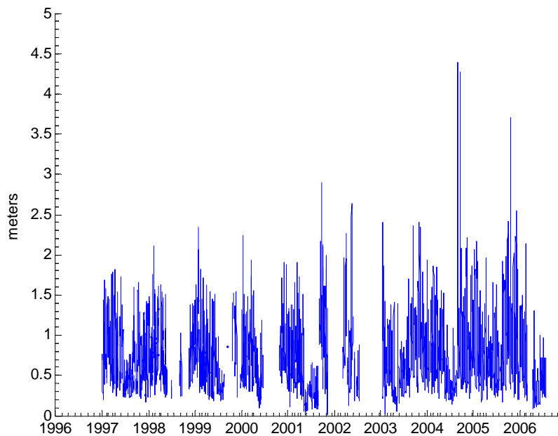
Figure 5. Significant Wave Height Data from Sebastian Inlet, FL (Harris and Flanary, 2007)
